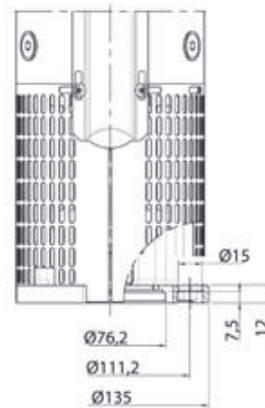
8" Motor Adapter
