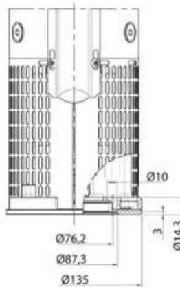
8" Motor Adapter
