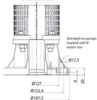
8" Motor Adapter
