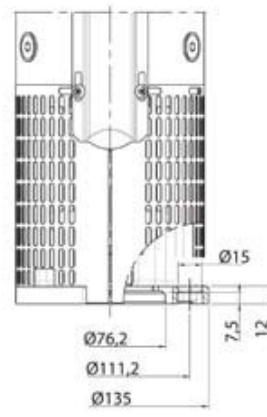
8" Motor Adapter
