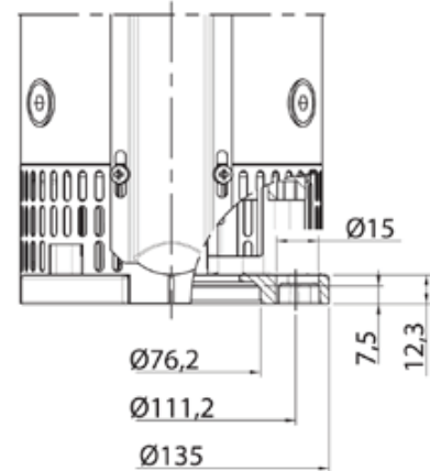
6" Motor Adapter
