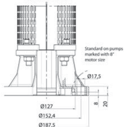
8" Motor Adapter
