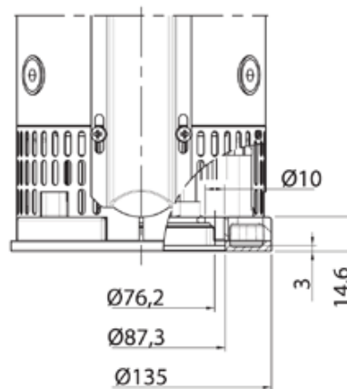
4" Motor Adapter
