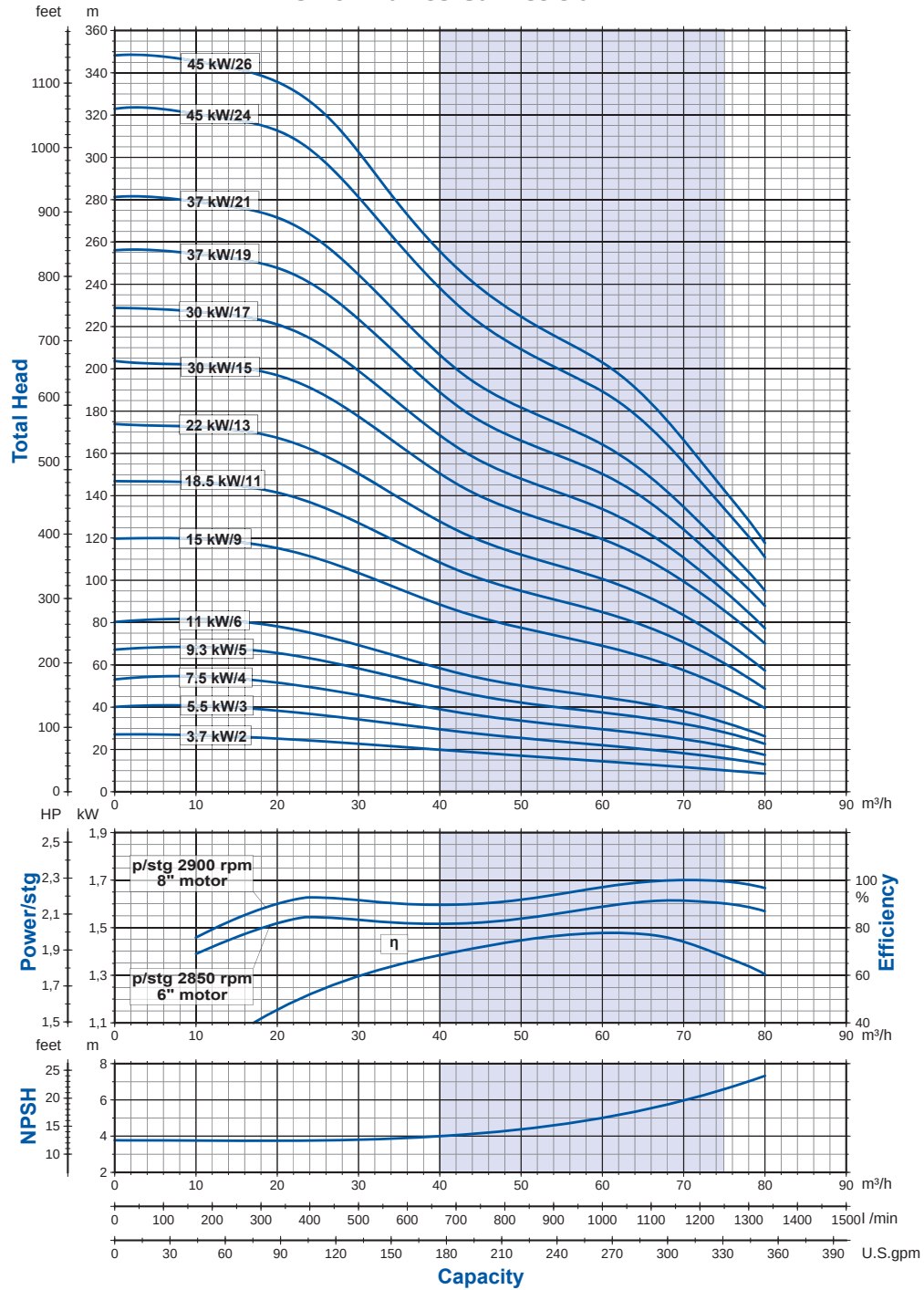
Performance Curves 50 Hz
